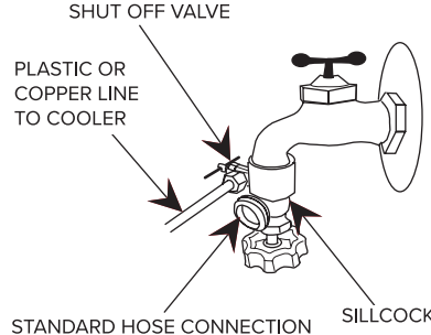
SILLCOCK CONNECTION
